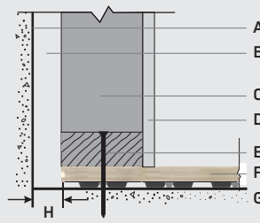
FIGURE 2 - Foundation Wall
